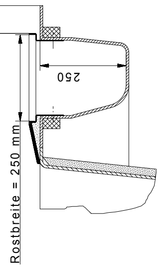
Detail X
